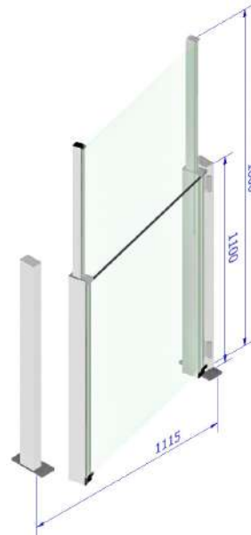
Wind Barrier with steel base
