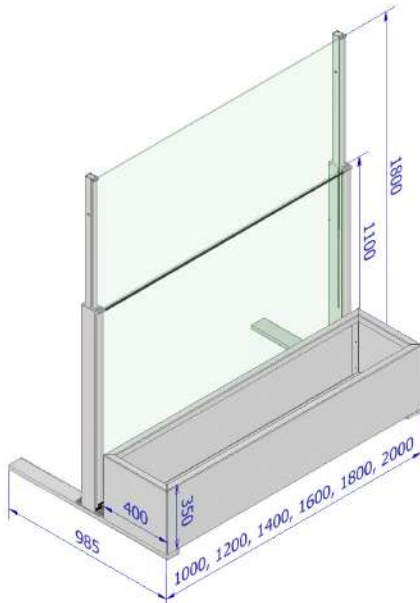
Wind Barrier with aluminium flowerpot
