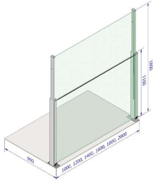
Wind Barrier with steel base
